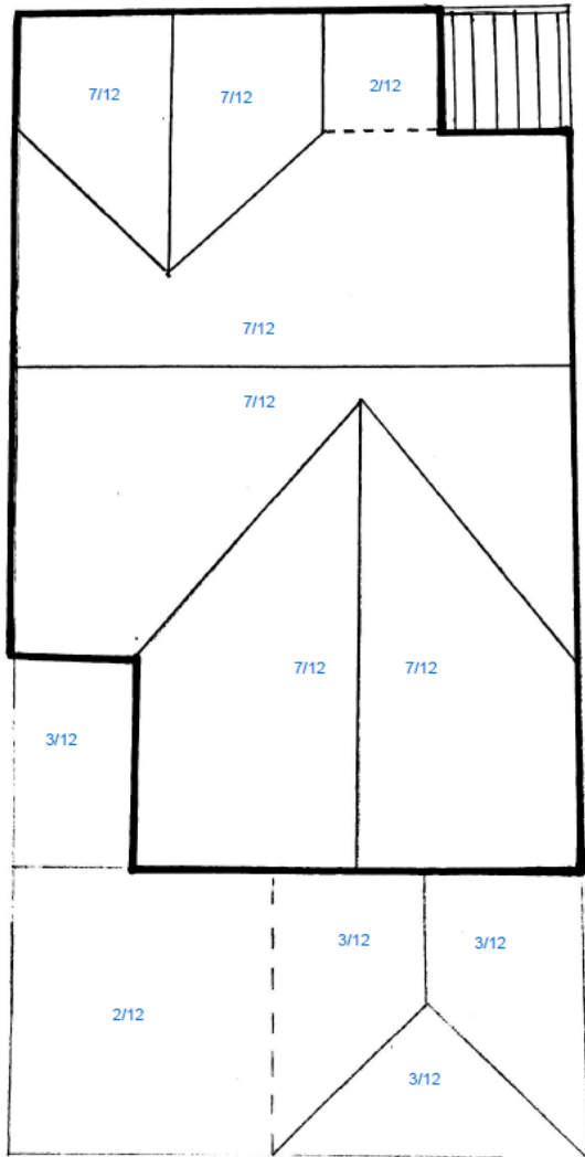
Figure 8 - Existing Roof Plan
